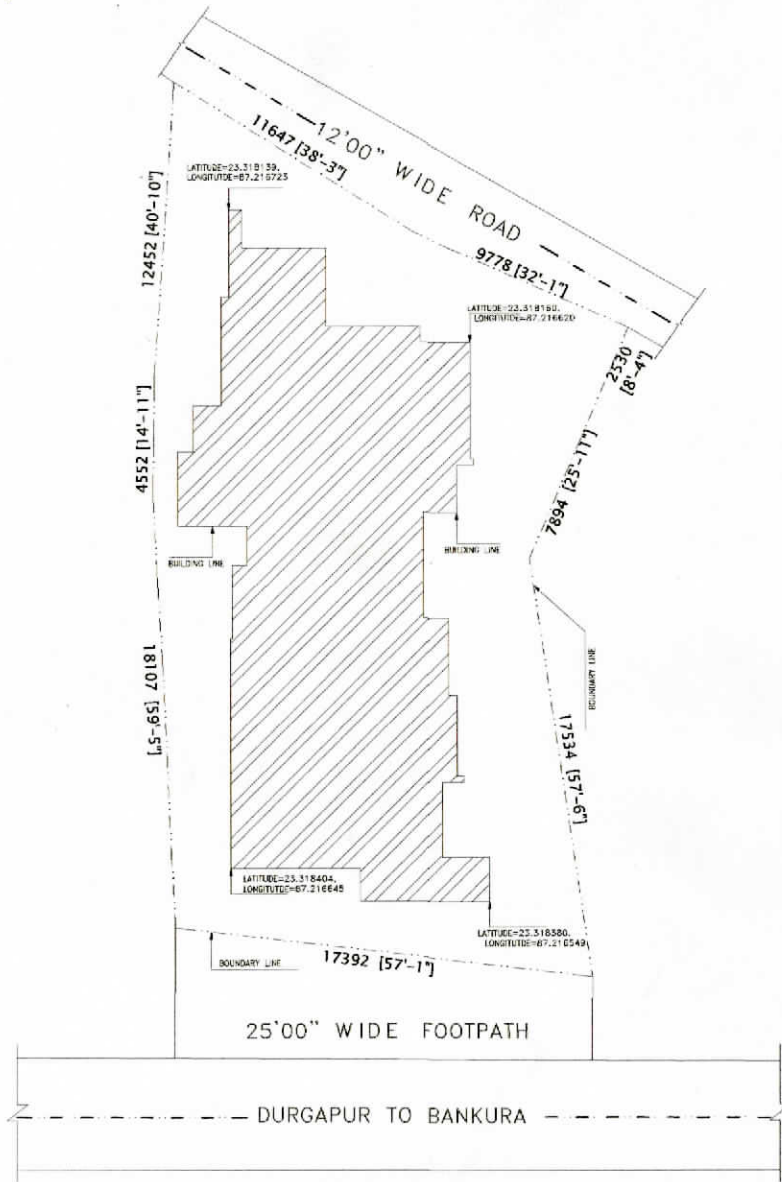
① SITE PLAN
